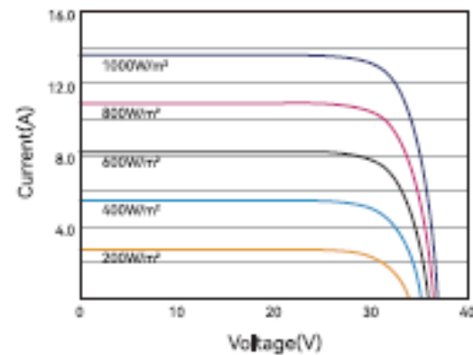
I-V Curves of PV Module (400W)
