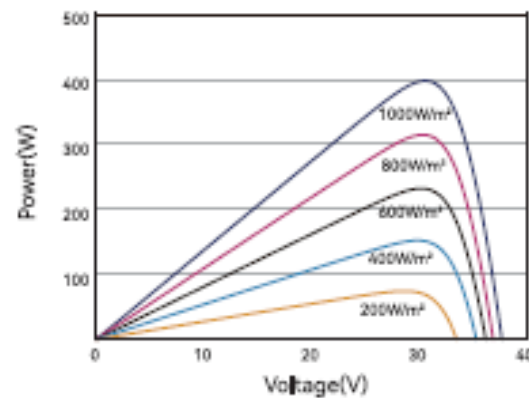
P-V Curves of PV Module (400W)
